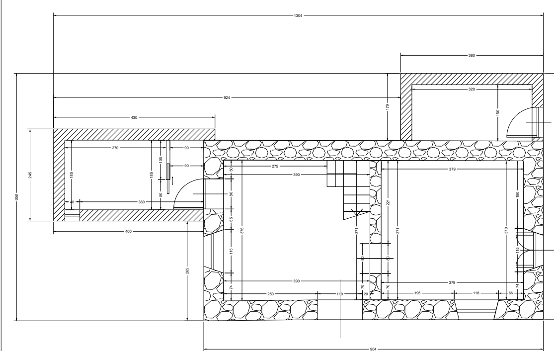
PIANO TERRA
