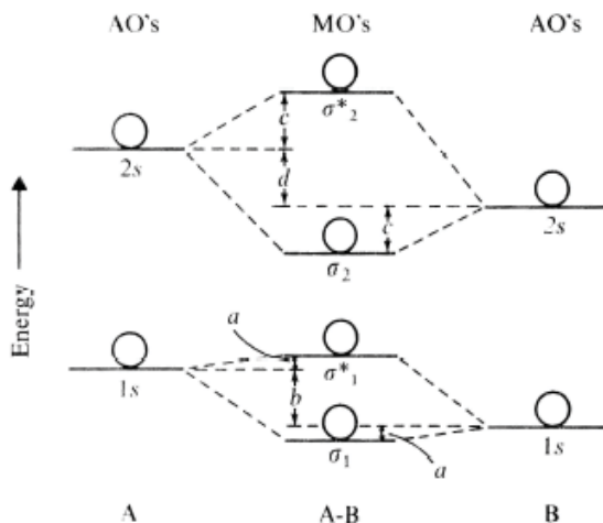
Figure 2.19 Molecular orbital diagram for an AB molecule.
