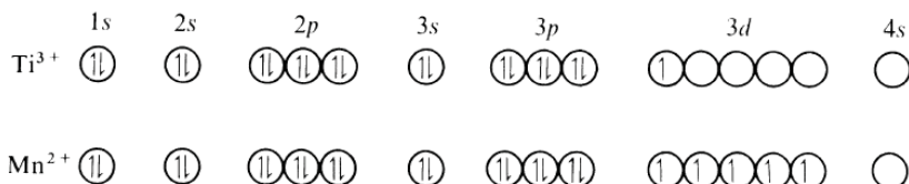
Figure 2.3 The electronic structures of \text{Ti}^{3+} and \text{Mn}^{2+} .
