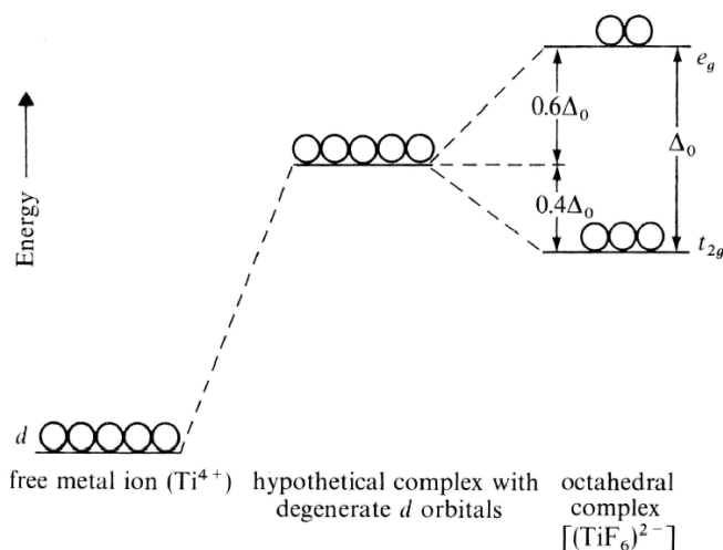
Figure 2.8 The energies of the d orbitals in a free metal ion, in a hypothetical complex in which there is no crystal field splitting, and in an octahedral complex.
