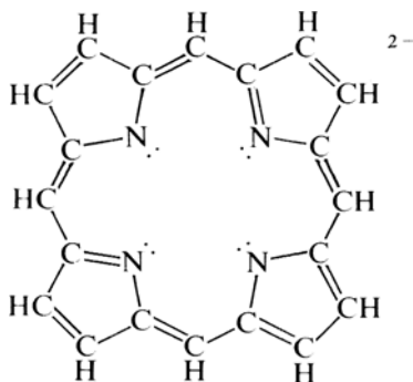
Porphine anion
