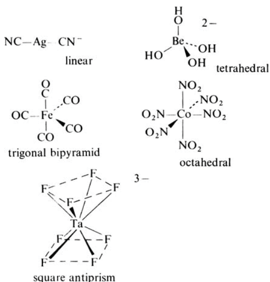
Figure 3.1 Illustrations of structures found in metal complexes.
