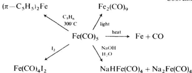
Figure 7.2 Reactions of \text{Fe(CO)}_5 illustrating reactions of metal carbonyls.
