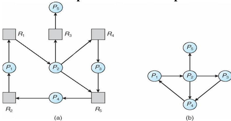
Resource-Allocation Graph
