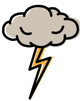
LIGHTNING
