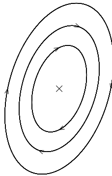
Fig. 29.7. Phase portrait for Exercise 29.1(vii).
