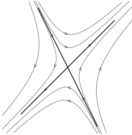
Fig. 31.1. The phase portrait for Exercise 31.1(i).
