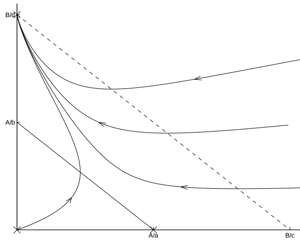
Fig. 33.31. The nullclines when A/b < B/d and A/a < B/c ( \dot{x} = 0 on solid line, \dot{y} = 0 on dashed line). Trajectories are attracted to (0, B/d) (case [Y]).
