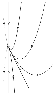
Fig. 33.9. The local phase portrait (0, 1) .
