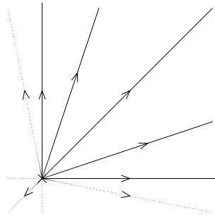
Fig. 33.1. The phase portrait near (0, 0) .
