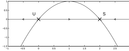
Fig. 7.2. The phase diagram for \dot{x} = x(2 - x) .
