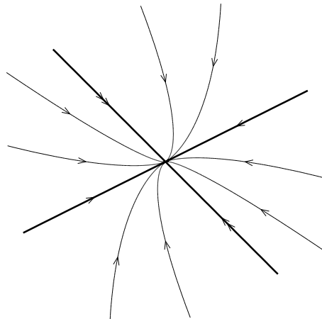
Fig. 31.4. The phase portrait for Exercise 31.1(iv).
