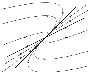
Fig. 28.7. The phase portrait for Exercise 28.1(vii).
