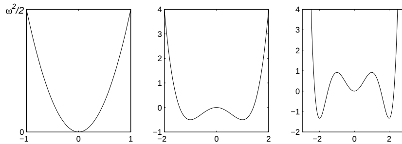
Fig. 34.1. From left to right, the potentials from parts (i), (ii), and (iii) of Exercise 34.1, plotted against x .
