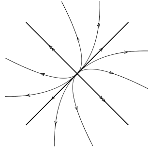
Fig. 28.1. The phase portrait for Exercise 28.1(i).
