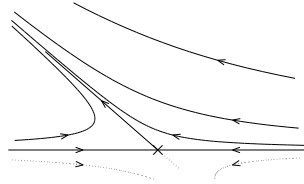
Fig. 33.5. The phase portrait near (2, 0) .
