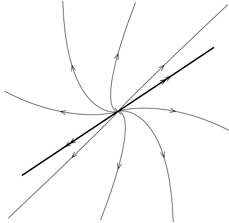
Fig. 31.3. The phase portrait for Exercise 31.1(iii).
