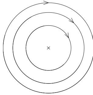
Fig. 34.2. The phase portrait for a particle in the potential V(x) = \frac{1}{2}\omega^2 x^2 .
