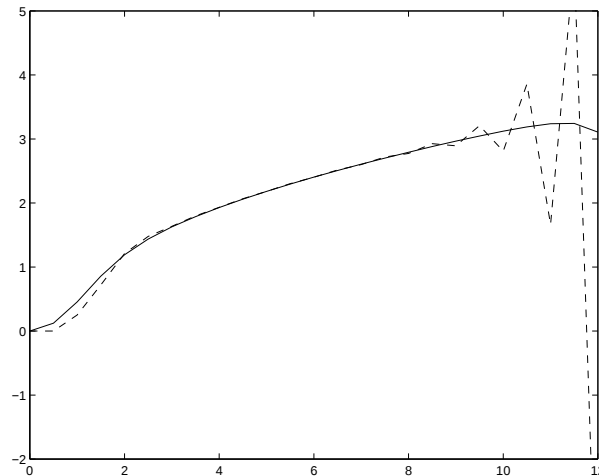
Fig. 21.3. The solution of \dot{x} = t - x^2 calculated using the fourth order Runge-Kutta scheme (solid line) and the Euler method (dashed line), both with h = \frac{1}{2} .
