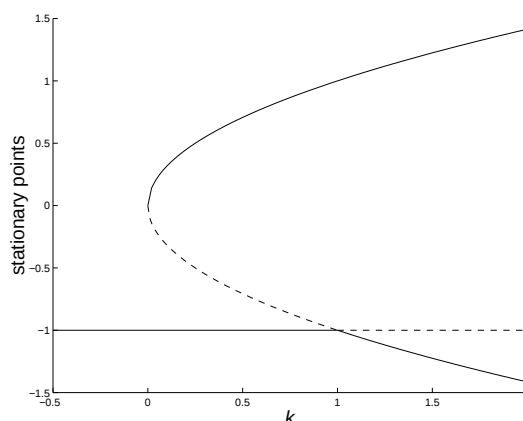
Fig. 7.16. The bifurcation diagram for the equation \dot{x} = -(1+x)(x^2 - k) [solid/dashed lines indicate stable/unstable stationary points]. There is a saddle-node bifurcation near x = 0 as k passes through zero, and a transcritical bifurcation near x = -1 and k passes through one.
