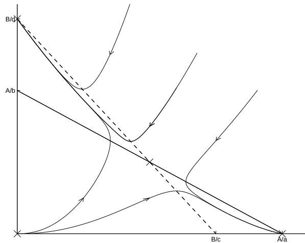
Fig. 33.32. The nullclines when A/b < B/d and A/a > B/c ( \dot{x} = 0 on solid line, \dot{y} = 0 on dashed line). In this case there are two possible attracting points, those on either axis (case [X/Y]).
