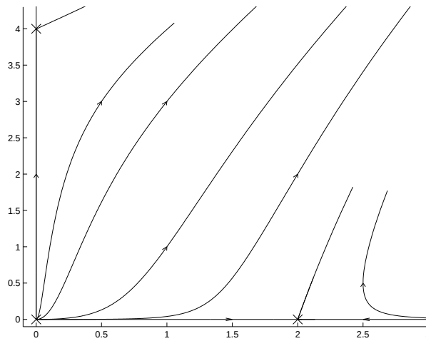
Fig. 33.30. For the cooperative system of Exercise 33.2(ii) both populations increase forever.
