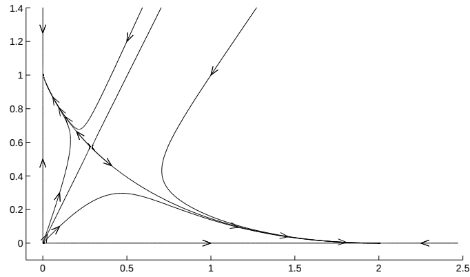
Fig. 33.12. The phase portrait for Exercise 33.1(iii).
