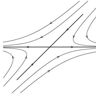
Fig. 28.2. The phase portrait for Exercise 28.1(ii).
