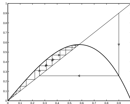
Fig. 24.2. The cobweb diagram for r = 1.5 . The new non-zero fixed point is now stable, and the origin is unstable.
