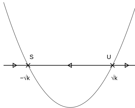
Fig. 7.12. The phase diagram for \dot{x} = x^2 - k when k is positive. There are two stationary points, a stable point at x = -\sqrt{k} and an unstable point at x = \sqrt{k} .
