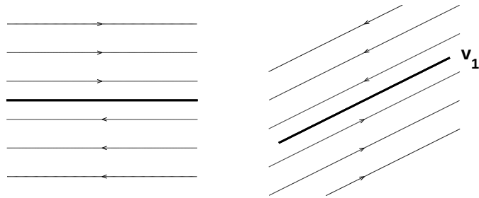
Fig. 30.6. Phase portraits for a repeated real eigenvalue zero with eigenvector \mathbf{v}_1 , in the transformed plane (left) and the original coordinates (right). In both cases the bold line consists entirely of stationary points.
