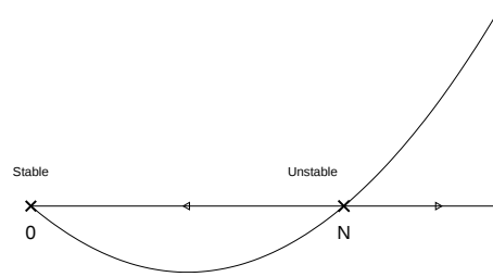
Fig. 7.9. The phase diagram for \dot{H} = -KH(N - H) : eventually there are no healthy members of the population left.
