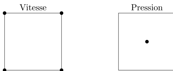
Figure 11.7 – Élément incompatible à pression discontinue Q_1 - Q_0
