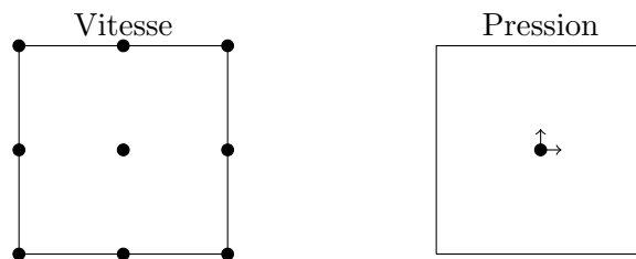
Figure 11.11 – Élément à pression discontinue Q_2 - P_1 ( O(h^2) )
