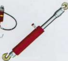
HJSD1303 10 Ton Pull Ram 732 mm Length 150 mm Stroke
