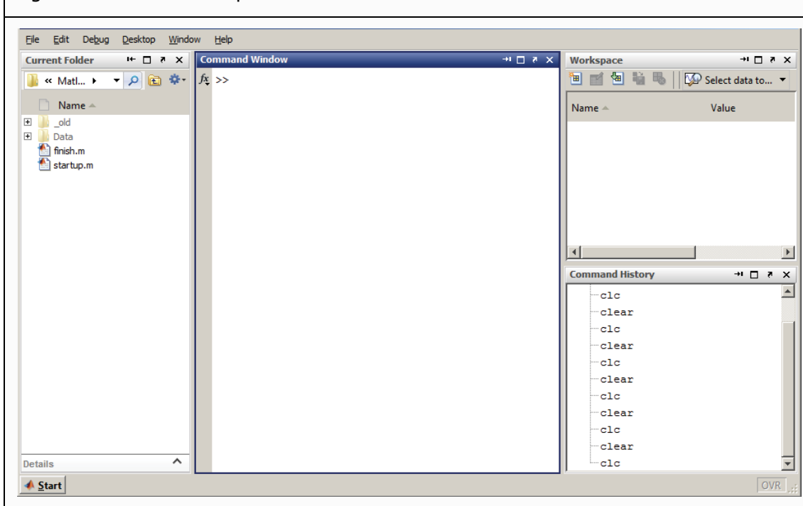
Figure 2-1: The Desktop
