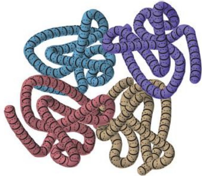
quaternary structure
