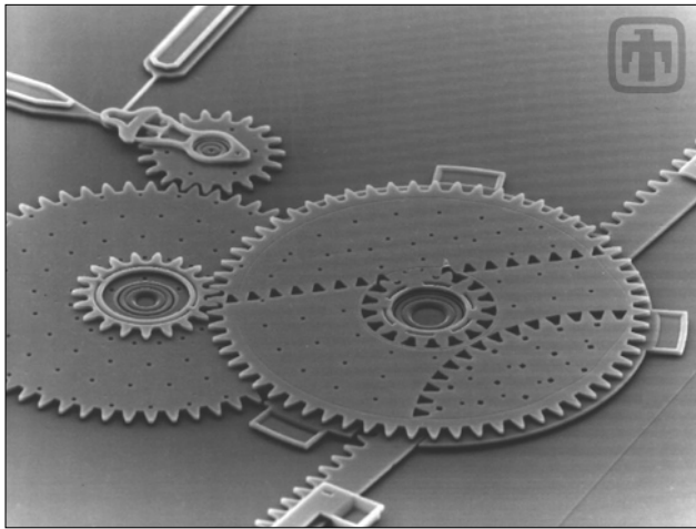
Figure 8-4: MEMS transmission to convert microengine output into linear motion.
