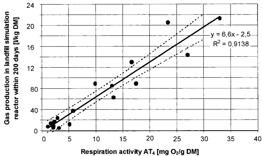
Fig. 6. Landfill gas production as a function of the stability parameter AT 4 [17]
