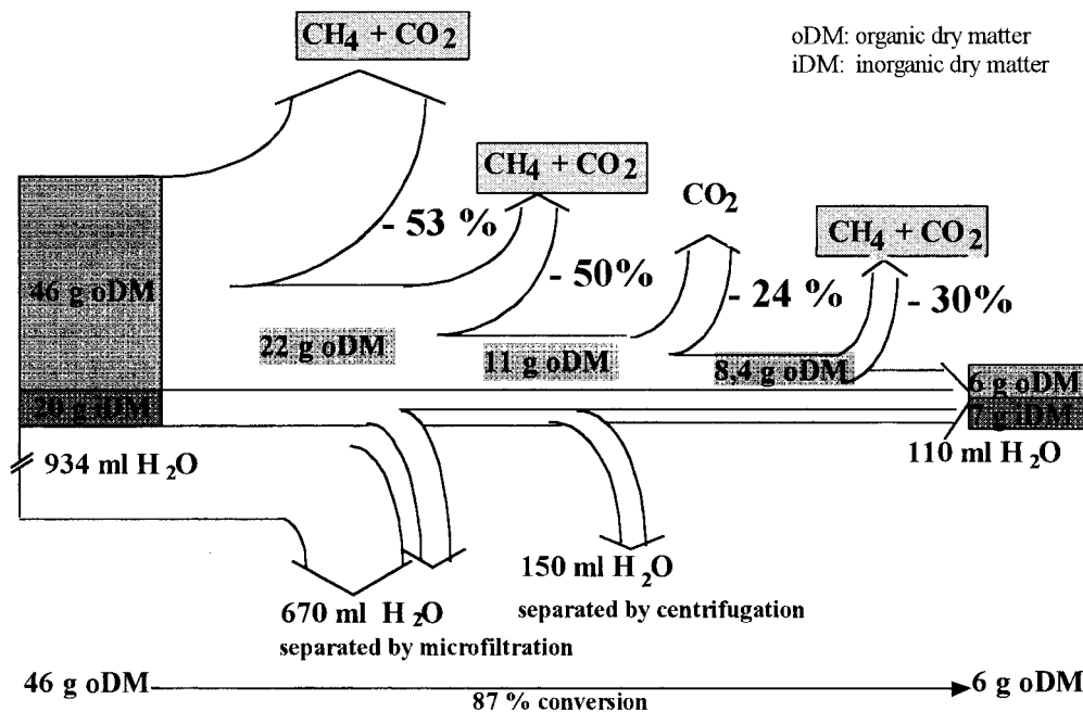
Fig. 3. Anaerobic degradation of waste components in a 4-stage alternating anaerobic/aerobic process [7]
