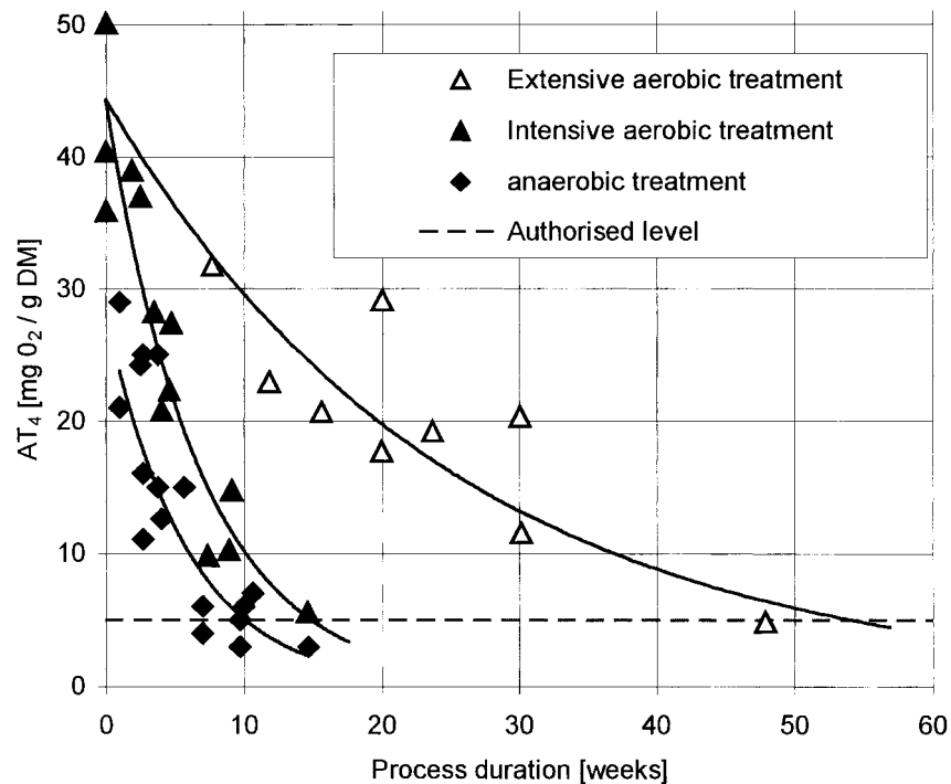
Fig. 5. Stability parameter AT_4 as a function of the treatment duration [2, p. 208]
