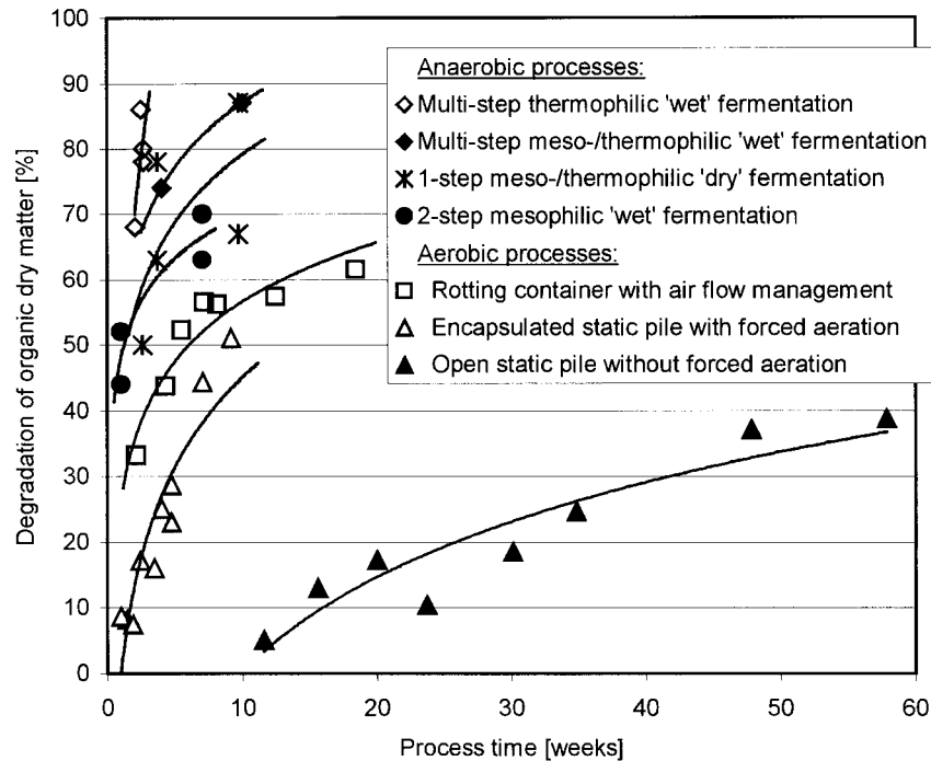
Fig. 4. Degradation of organic matter by different anaerobic and aerobic processes [2]
