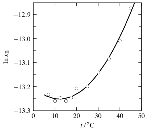
Figure 12.8 Aqueous solubility of liquid n -butylbenzene as a function of temperature (Ref. [125]).
