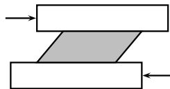
Figure 2.1 Experimental procedure for producing shear stress in a phase (shaded). Blocks at the upper and lower surfaces of the phase are pushed in opposite directions, dragging the adjacent portions of the phase with them.
