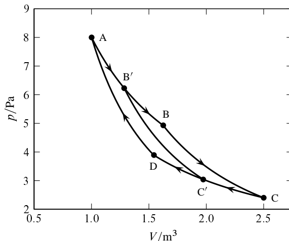
Figure 4.3 Indicator diagram for a Carnot engine using an ideal gas as the working substance. In this example, T_h = 400\text{ K} , T_c = 300\text{ K} , \epsilon = 1/4 , C_{V,m} = (3/2)R , n = 2.41\text{ mmol} . The processes of paths A \rightarrow B and C \rightarrow D are isothermal; those of paths B \rightarrow C , B' \rightarrow C' , and D \rightarrow A are adiabatic. The cycle A \rightarrow B \rightarrow C \rightarrow D \rightarrow A has net work w = -1.0\text{ J} ; the cycle A \rightarrow B' \rightarrow C' \rightarrow D \rightarrow A has net work w = -0.5\text{ J} .
