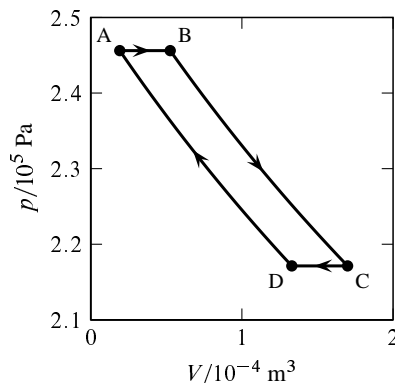
Figure 4.4 Indicator diagram for a Carnot engine using \text{H}_2\text{O} as the working substance. In this example, T_h = 400\text{ K} , T_c = 396\text{ K} , \epsilon = 1/100 , w = -1.0\text{ J} . In state A, the system consists of one mole of \text{H}_2\text{O}(l) . The processes (all carried out reversibly) are: A \rightarrow B , vaporization of 2.54\text{ mmol H}_2\text{O} at 400\text{ K} ; B \rightarrow C , adiabatic expansion, causing vaporization of an additional 7.68\text{ mmol} ; C \rightarrow D , condensation of 2.50\text{ mmol} at 396\text{ K} ; D \rightarrow A , adiabatic compression returning the system to the initial state.
