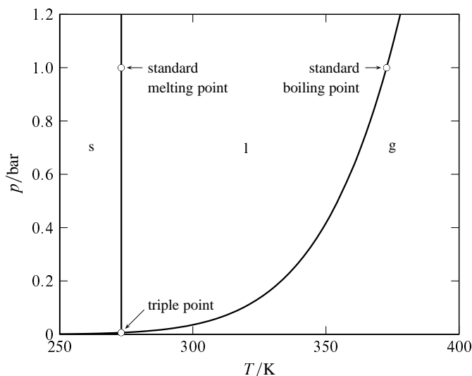
Figure 8.6 Pressure–temperature phase diagram of \text{H}_2\text{O} . (Based on data in Ref. [124].)
