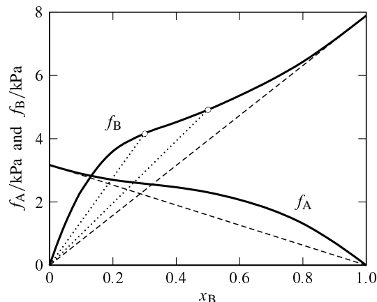
Figure 12.10 Fugacities in a gas phase equilibrated with a binary liquid mixture of H 2 O (A) and ethanol (B) at 25 °C and 1 bar. a The dashed lines show Raoult's law behavior. The dotted lines illustrate the inequality (df_B/dx_B) < (f_B/x_B) .
