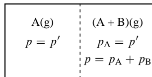
Figure 9.4 System with two gas phases, pure A and a mixture of A and B, separated by a semipermeable membrane through which only A can pass. Both phases are ideal gases at the same temperature.
