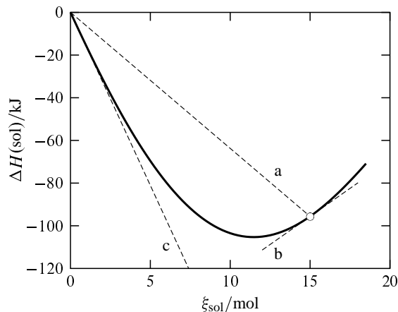
Figure 11.9 Enthalpy change for the dissolution of \text{NaCH}_3\text{CO}_2(\text{s}) in one kilogram of water in a closed system at 298.15 K and 1 bar, as a function of the amount \xi_{\text{sol}} of dissolved solute. a The open circle at \xi_{\text{sol}}=15 mol indicates the approximate saturation limit; data to the right of this point come from supersaturated solutions. At the composition m_{\text{B}}=15 mol \text{kg}^{-1} , the value of \Delta H_{\text{m}}(\text{sol}, m_{\text{B}}) is the slope of line a and the value of \Delta_{\text{sol}}H is the slope of line b. The value of \Delta_{\text{sol}}H^\infty is the slope of line c.
