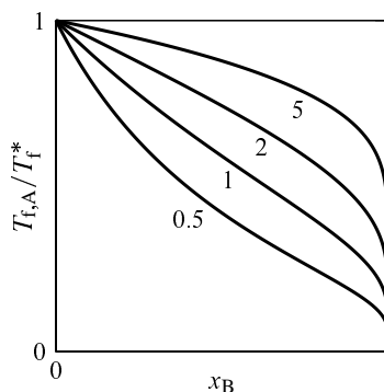
Figure 12.5 Freezing-point curves of ideal binary liquid mixtures. The solid is component A. Each curve is calculated from Eq. 12.5.4 and is labeled with the value of \Delta_{\text{fus,A}}H/RT_{f,A}^* .
