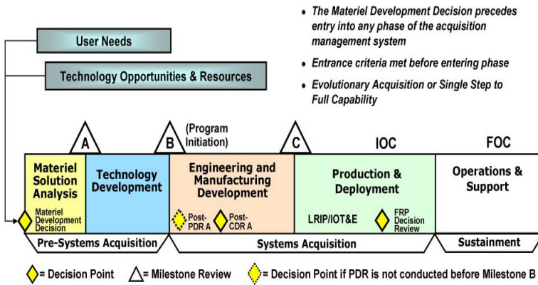
Figure 3. Acquisition Milestones
