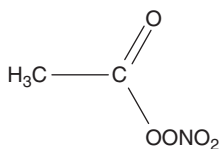
Peroxyacetyl nitrate
