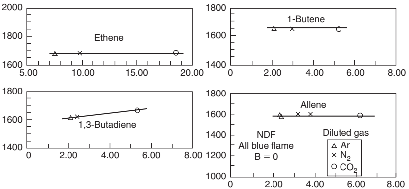
FIGURE 8.16 Incipient soot formation temperature as a function of the amount of diluent. The ordinate is the temperature in kelvins; the abscissa is f = (Q_f/Q_f + Q_{dg}) \times 100 , where Q_f is the volumetric flow rate of the fuel and Q_{dg} is that of the diluent.
