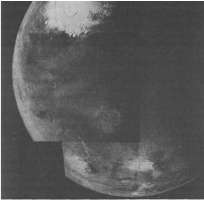
Mariner 9 composite photograph of Mars. Great volcanoes are seen at the bottom, the northern polar cap at the top. The amount of carbon dioxide and water frost locked in the polar cap, if released into the atmosphere, would probably produce much more Earth-like climatic conditions. Courtesy, NASA.
