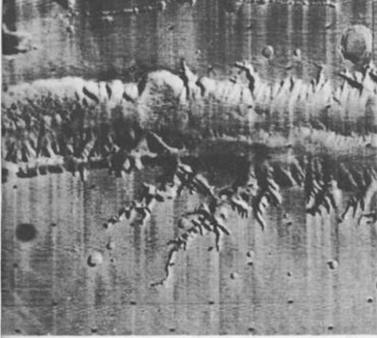
The great Coprates Rift Valley. Courtesy, NASA.
