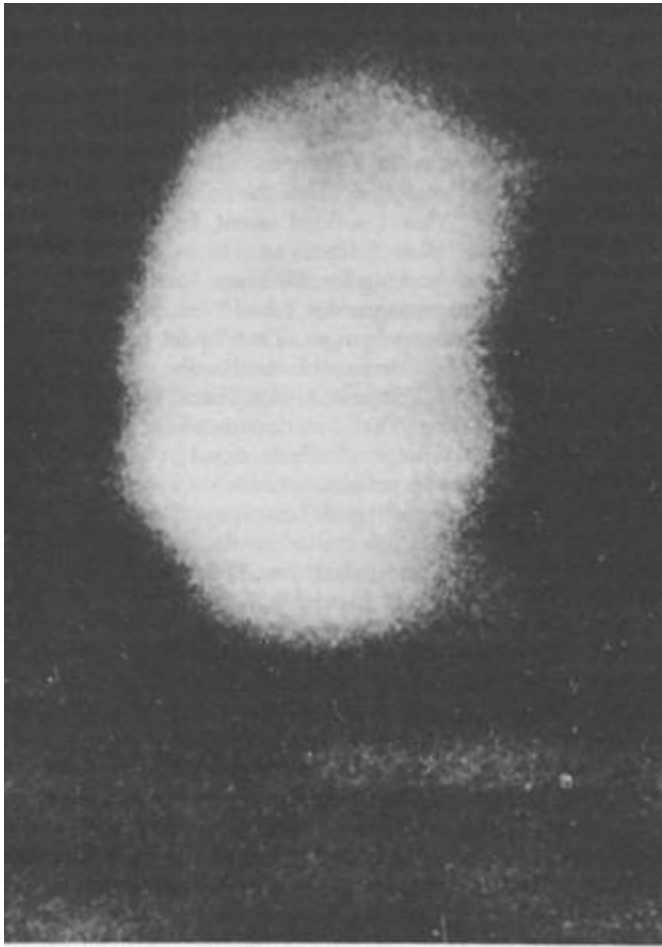
The first Mariner 9 image of Phobos, unprocessed by computer. (See also photos on pages 102 and 103.)
