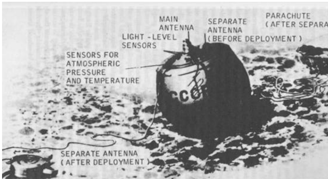
Sketch of the Venera 8 spacecraft, landed on the surface of Venus in 1972. From Tass.
