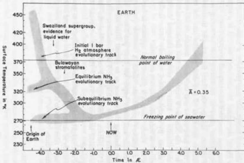
Schematic temperature evolutionary tracks of the planet Earth through geological time. The temperature changes shown are driven by changes in the Sun's luminosity and the composition of the Earth's atmosphere. One aeon is a billion years. From calculations by the author. Courtesy, American Association for the Advancement of Science.
