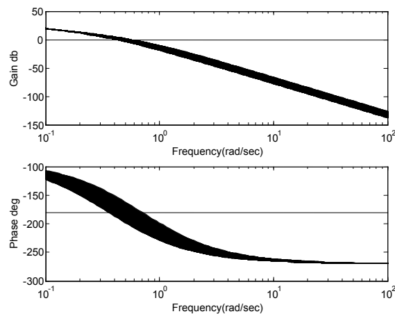
Figure 9.9 Stability from the Bounds of the Bode plots.
