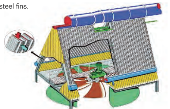
Typical ACC module
