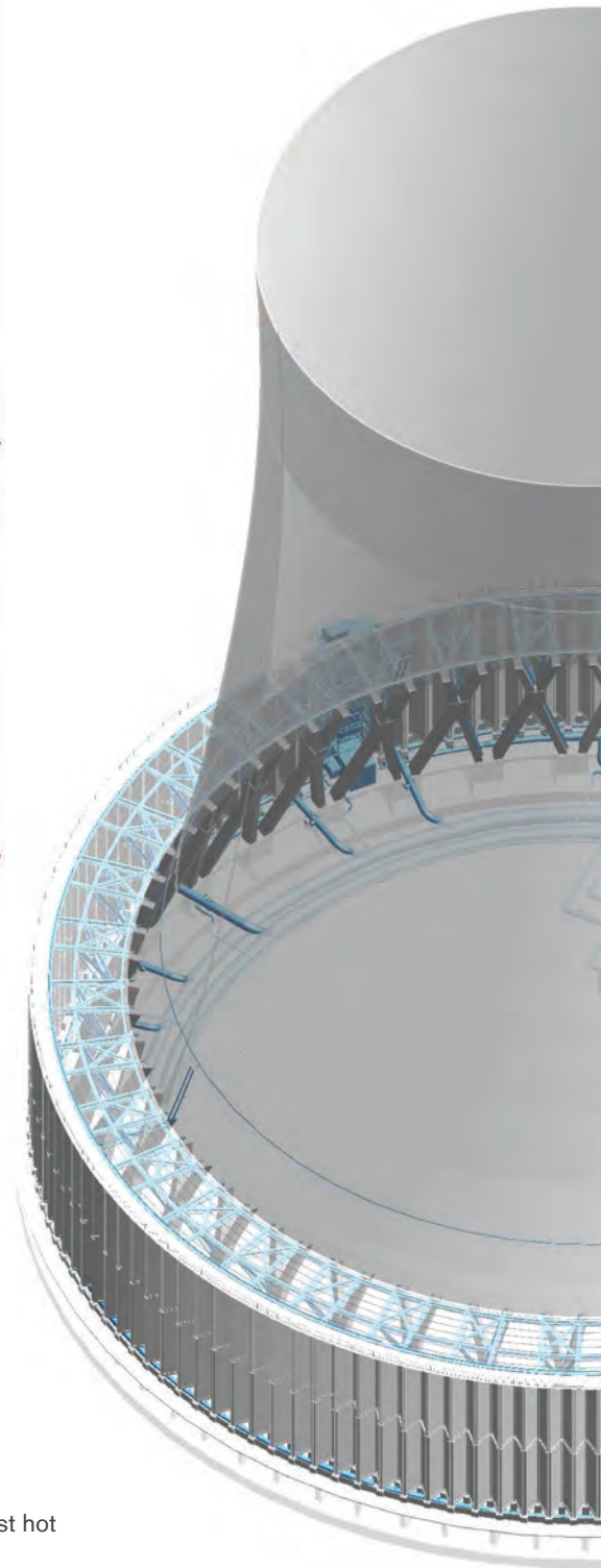
MegaDelta with louvers and piping
